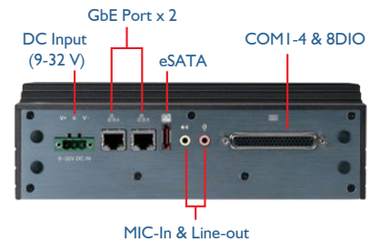
MXE-5400 Series Back Panel
