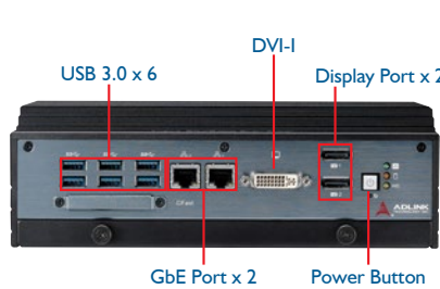
MXE-5400 Series Front Panel
