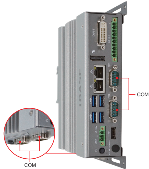
4x serial ports (RS232/422/485)
